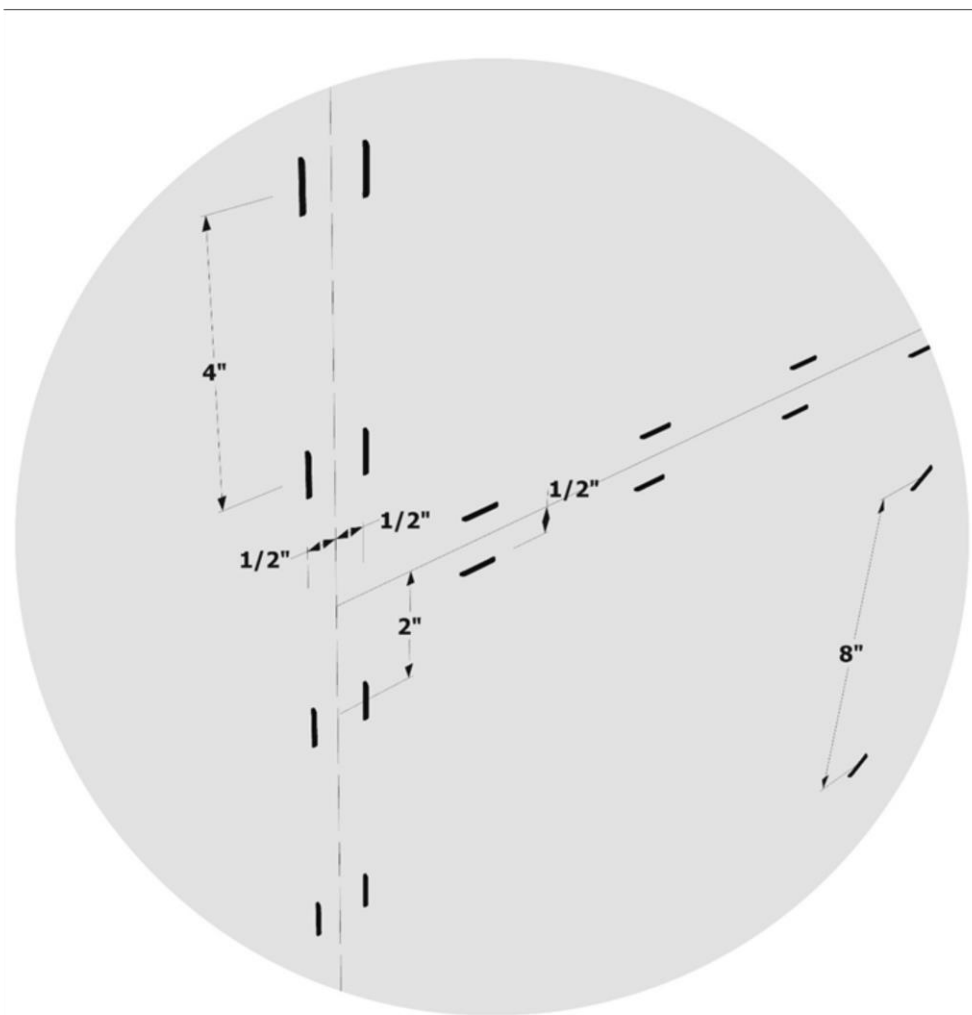
Fig 3. Mounting with Staples
