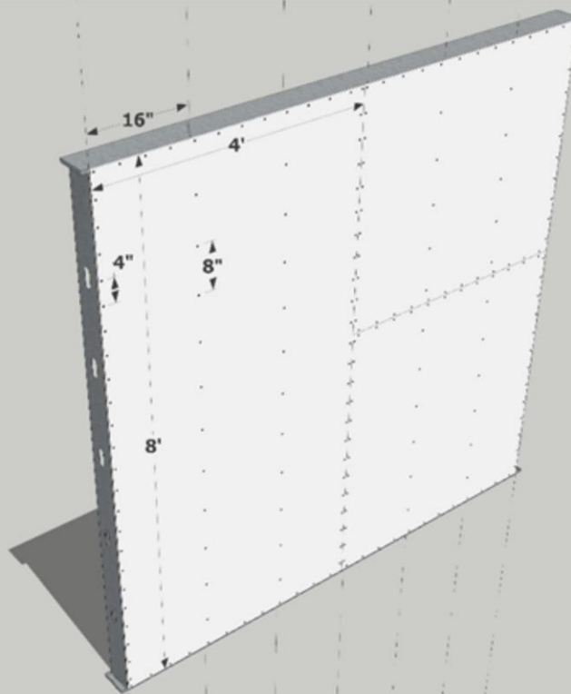
Fig 2. E72 GREENEXBOARD-Exterior sheathing 1/2" installed on 1 5/8" x 3.5" 18 Gauge Galvanized Steel Framing.
